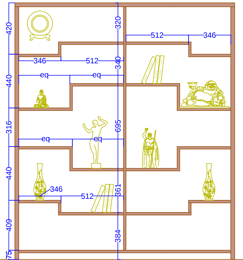
Internal Elevation
